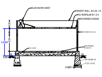
SECTION ON-'AB'
