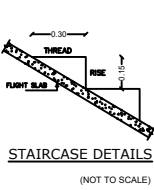
STAIRCASE DETAILS
