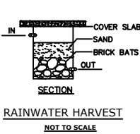
RAINWATER HARVEST
