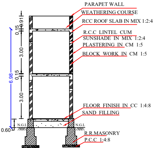
SECTION ON-'AB'
