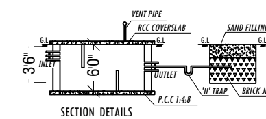
SECTION DETAILS
