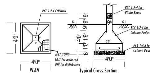
FOOTING DETAILS
