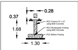
SUBSTRUCTURE DETAILS
