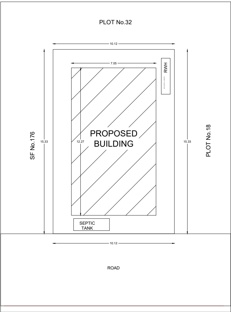
KEY PLAN
