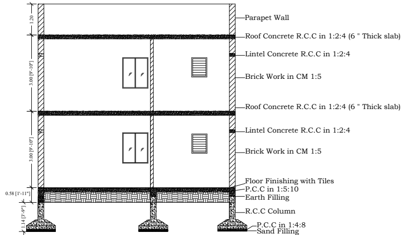
SECTION X-X
