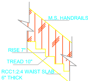
STAIRCASE DETAILS SCALE- 1:20
