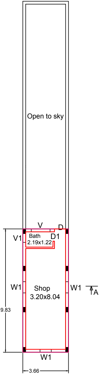
PLAN - First Floor
