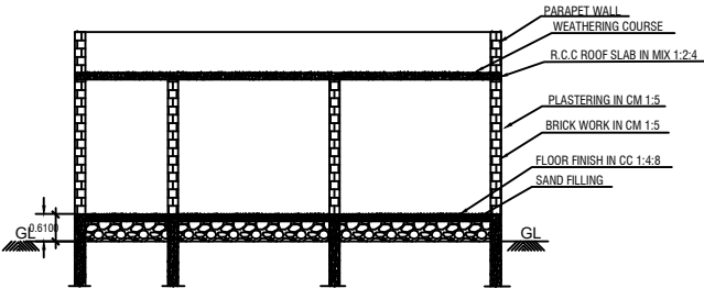
SECTION ON "MA"
