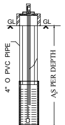
SECTION OF BORE WELL
