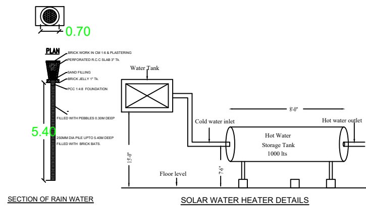
SECTION OF RAIN WATER PERCOLATION PIT
