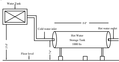
SOLAR WATER HEATER DETAILS
