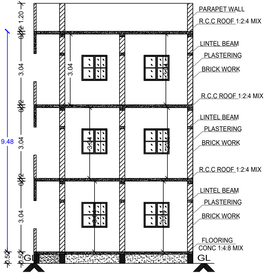
SECTION : "A-B"
