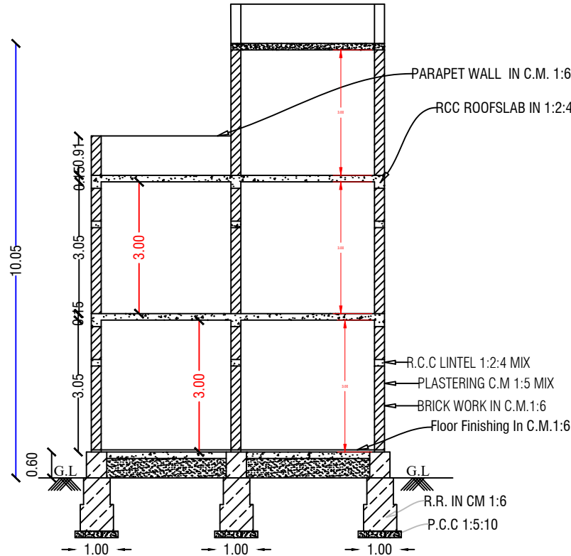
SECTION ON-\"AB\"
