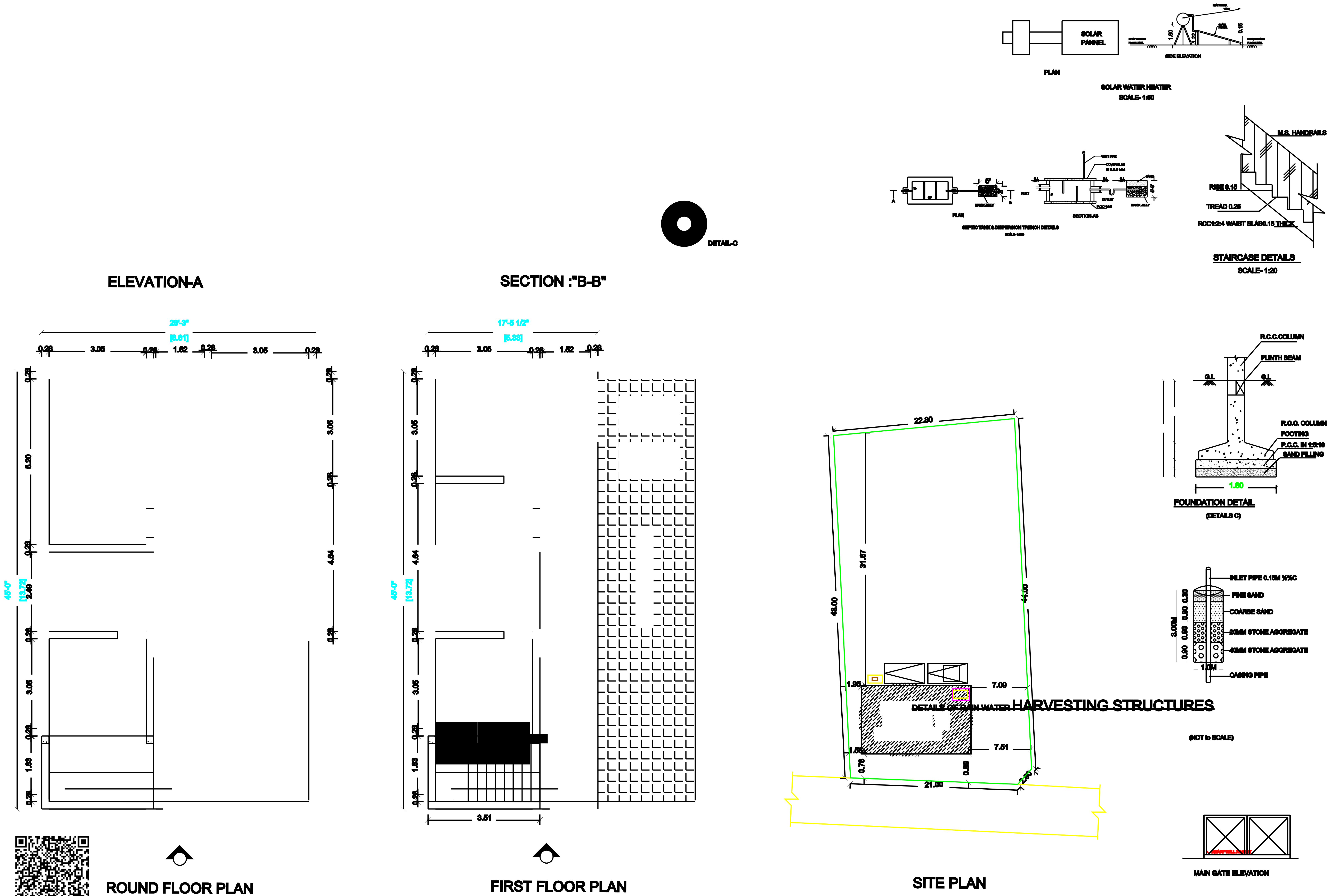
ROUND FLOOR PLAN
