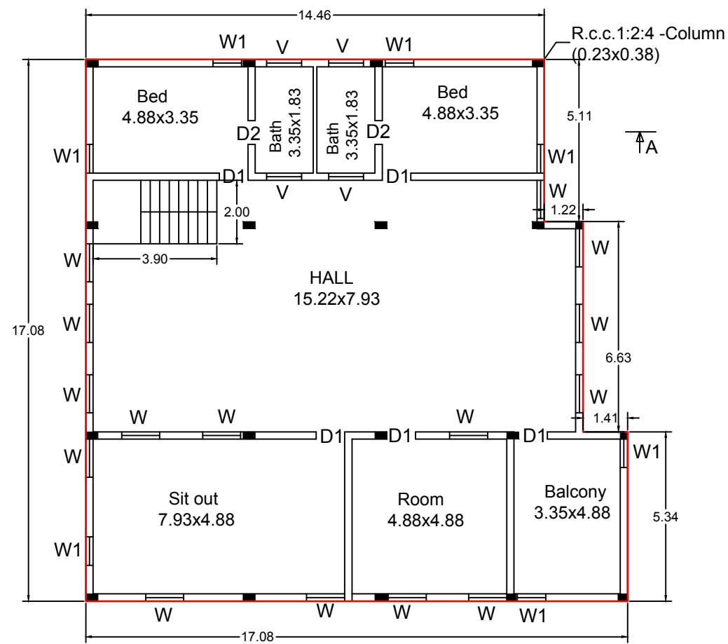
PLAN - First Floor
