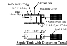
Septic Tank with Dispersion Trench
