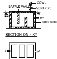
SEPTICTANK DETAILS NOT TO SCALE
