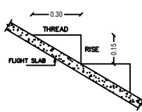
STAIRCASE DETAILS (NOT TO SCALE)
