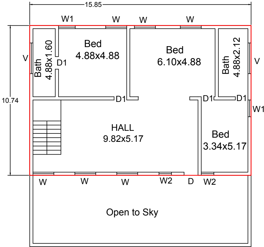
PLAN - First Floor
