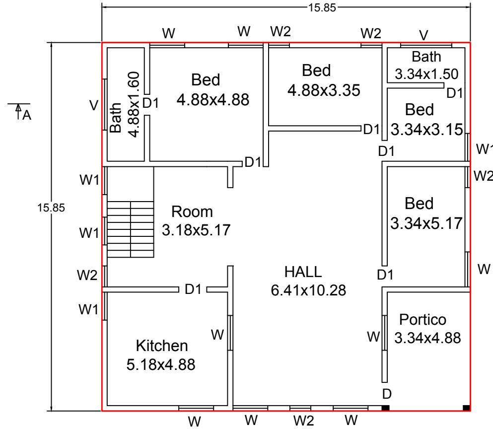
PLAN - Ground Floor
