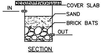
RAINWATER HARVEST NOT TO SCALE
