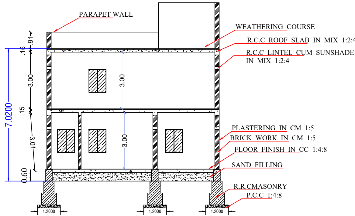
SECTION ON-"AB"
