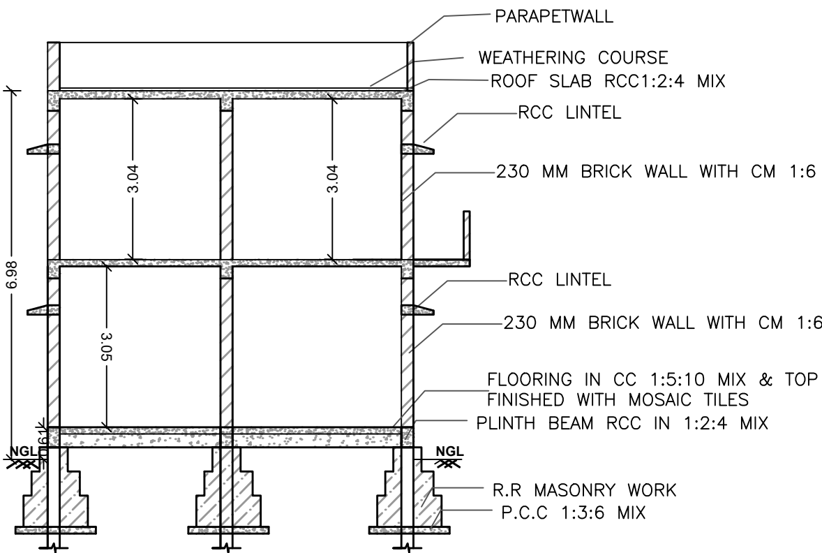
SECTION : "B-B"
