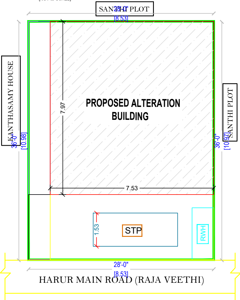
SITE PLAN FOR PROPOSED ALTERATION BUILDING (Scale 1:100)
