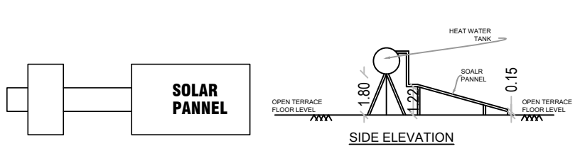
SOLAR WATER HEATER SCALE- 1:50
