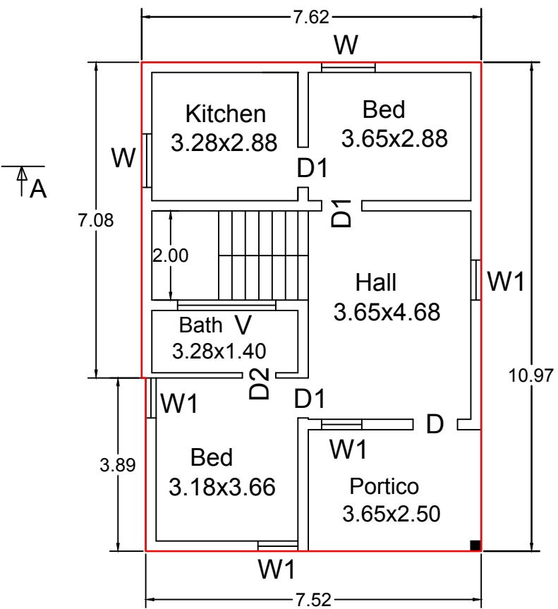
PLAN - Ground Floor
