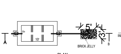
SEPTIC TANK & DISPERSION TRENCH DETAILS SCALE- 1:100
