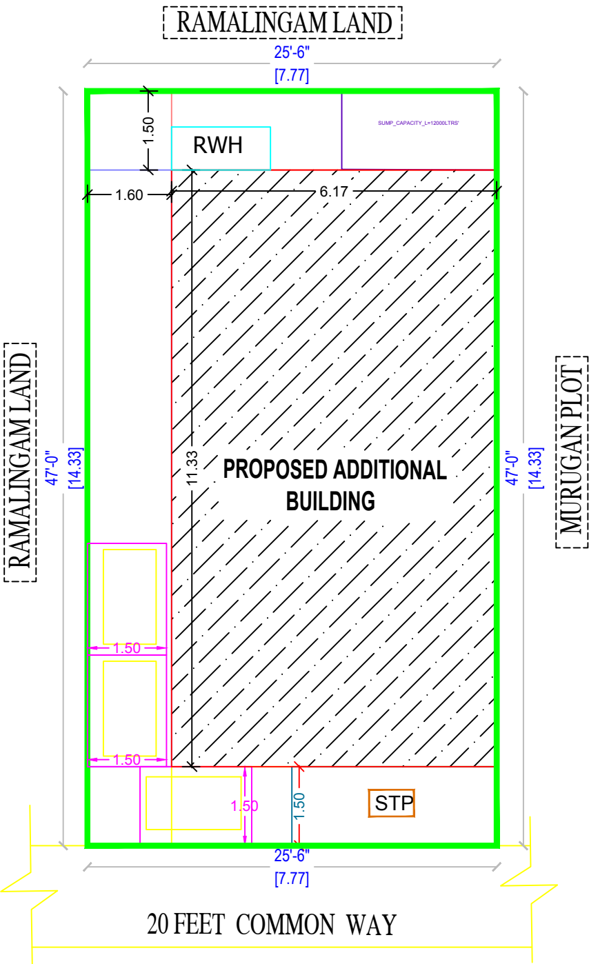
SITE PLAN FOR PROPOSED ADDITIONAL BUILDING
