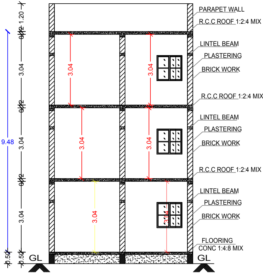
SECTION : "A-B"
