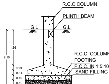
FOUNDATION DETAIL (DETAILS C)
