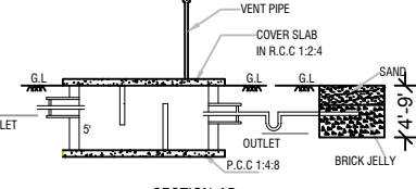
SEPTIC TANK & DISPERSION TRENCH DETAILS SCALE- 1:100
