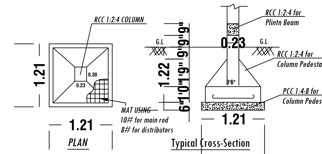
FOOTING DETAILS
