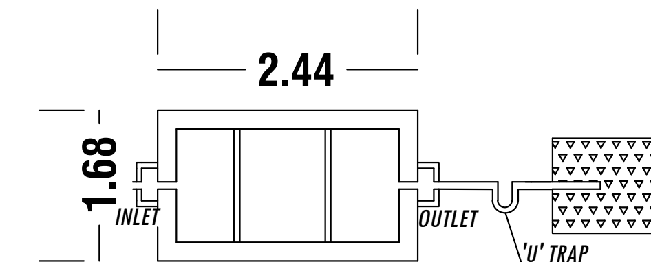
PLAN SEPTIC TANK AND DISPERSION TRENCH DETAILS
