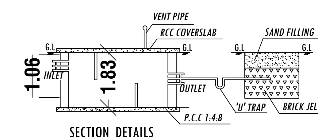
SECTION DETAILS
