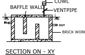
SECTION ON - XY PLAN SEPTICTANK DETAILS NOT TO SCALE
