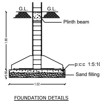
FOUNDATION DETAILS
