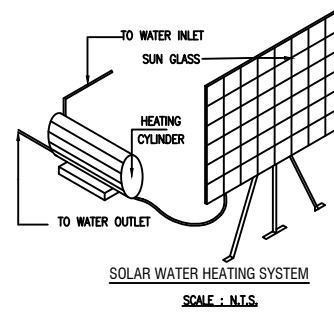
SOLAR WATER HEATING SYSTEM SCALE : N.T.S.
