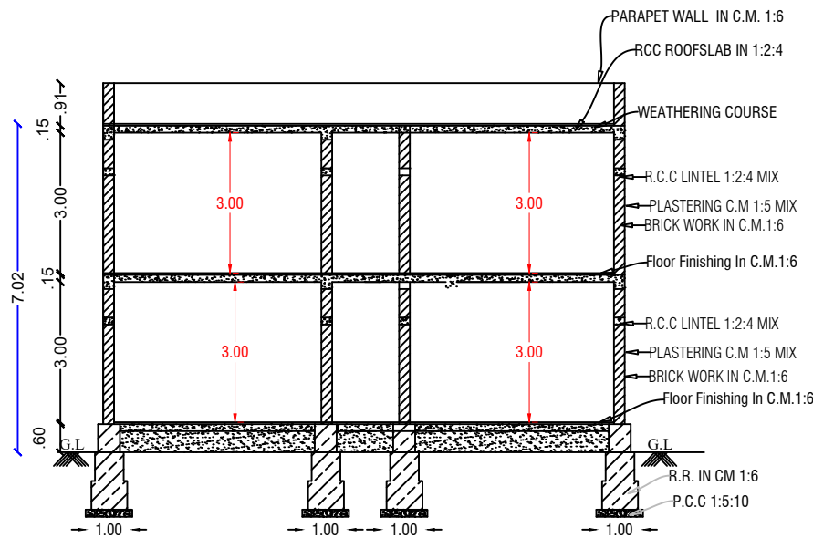
SECTION ON-'AB'
