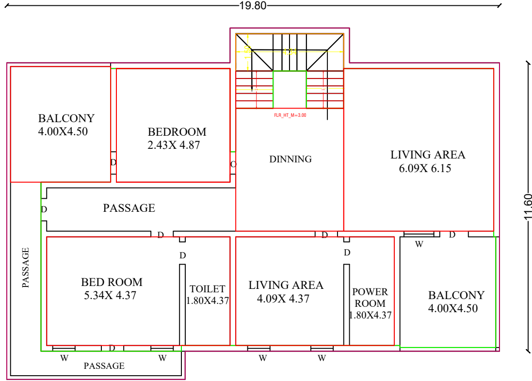
FRIST FLOOR PLAN
