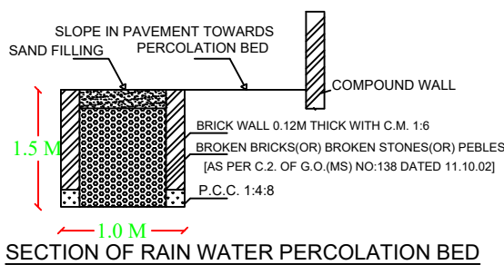
SECTION OF RAIN WATER PERCOLATION BED
