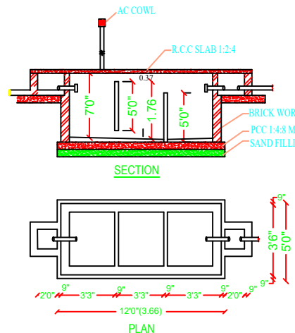
SECTION
