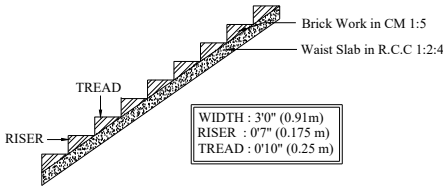
STAIRCASE DETAILS
