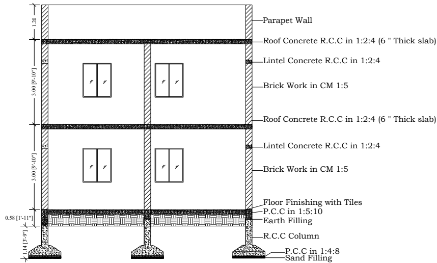
SECTION X-X
