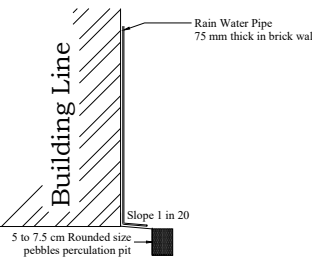
RAINWATER HARVESTING
