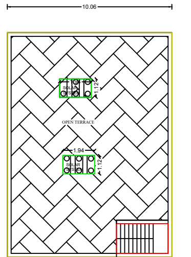
TERRACE PLAN
