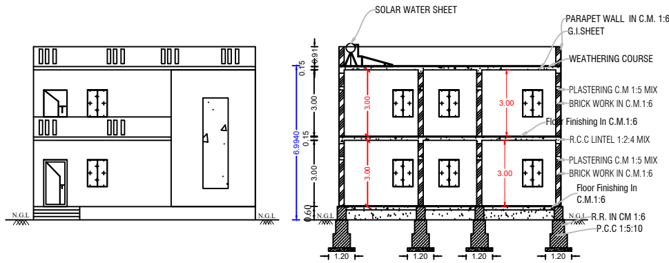
FRONT ELEVATION
