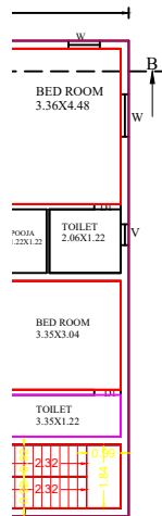
FIRST FLOOR PLAN
