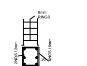
COLUMN DETAILS
