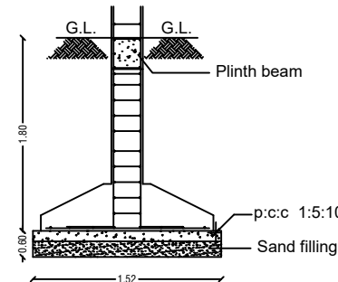
FOUNDATION DETAILS
