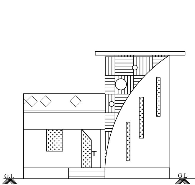
FRONT ELEVATION
