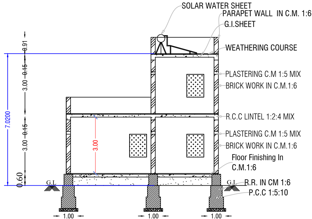
SECTION ON-"AB"
