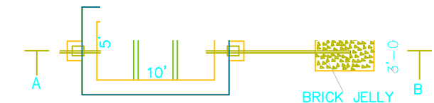
SEPTIC TANK & DISPERSION TRENCH DETAILS SCALE- 1:100
