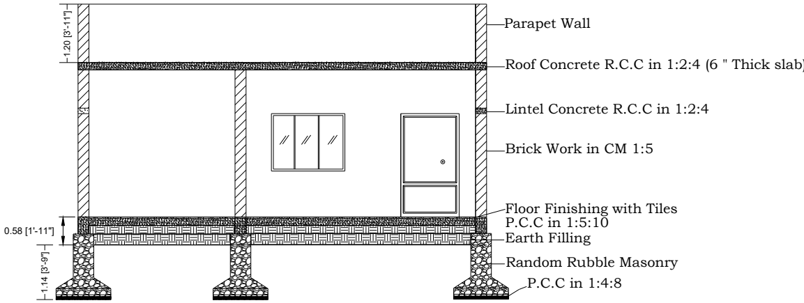
SECTION X-X
