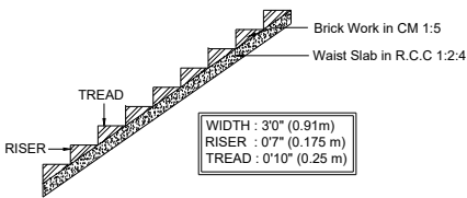
STAIRCASE DETAILS
