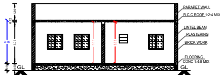
SECTION : "A-B"
