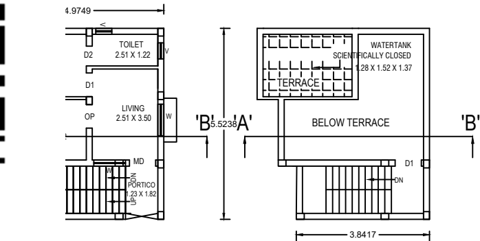
EXT. FIRST FLOOR PLAN.
