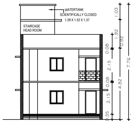
FRONT ELEVATION.
