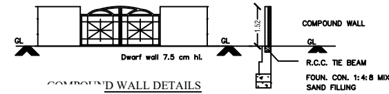
SECTION
