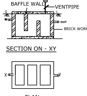
SEPTICTANK DETAILS NOT TO SCALE
