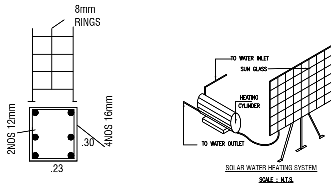
COLUMN DETAILS (NOT TO SCALE)
