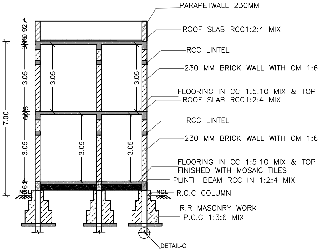
SECTION : "B-B"
