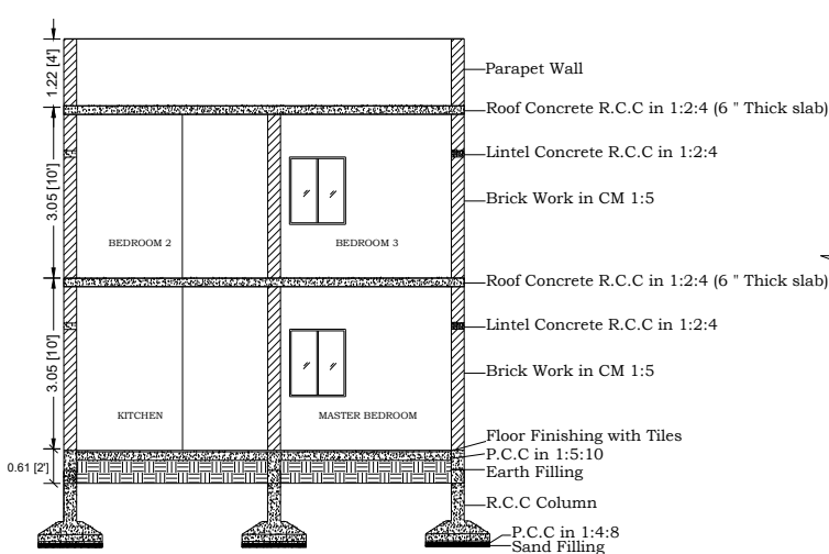
SECTION X-X
