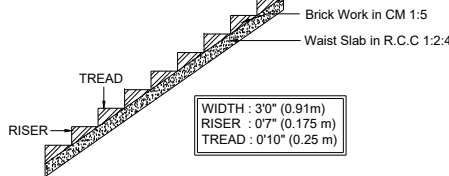
STAIRCASE DETAILS
