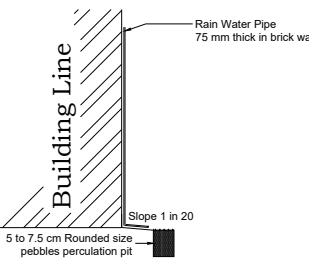
RAINWATER HARVESTING
