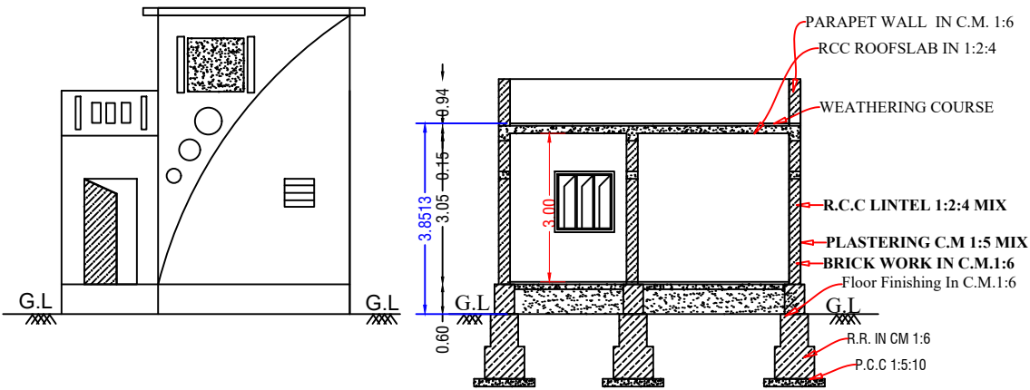
Elevation Plan
