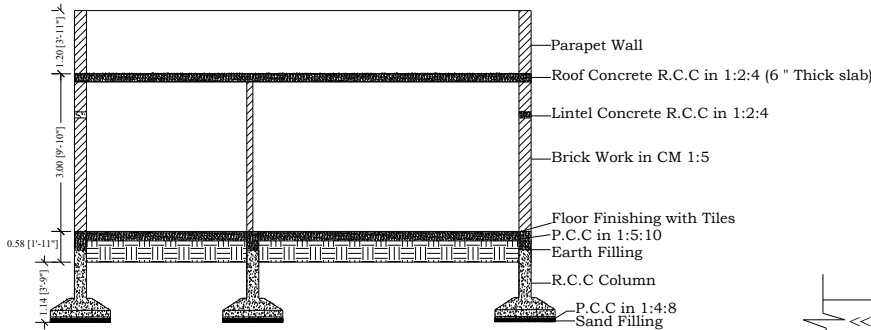
SECTION X-X
