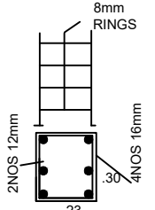
COLUMN DETAILS (NOT TO SCALE)
