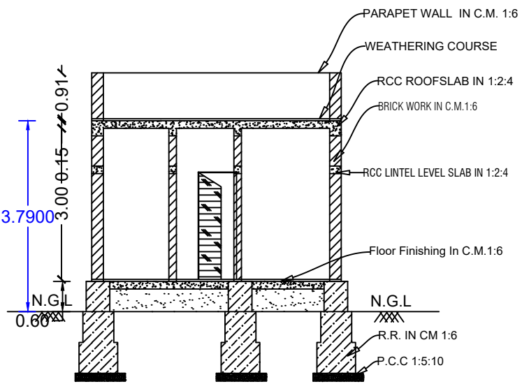
SECTION ON-"AB"
