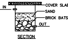
RAINWATER HARVEST NOT TO SCALE
