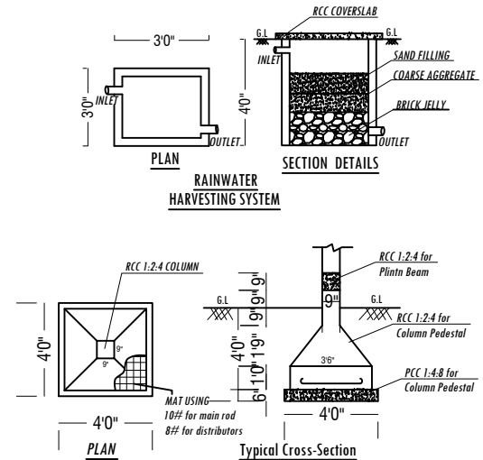
FOOTING DETAILS
