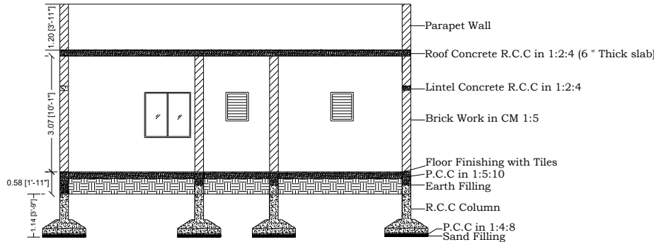
SECTION X-X
