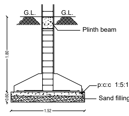
FOUNDATION DETAILS
