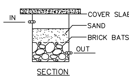
RAINWATER HARVEST NOT TO SCALE
