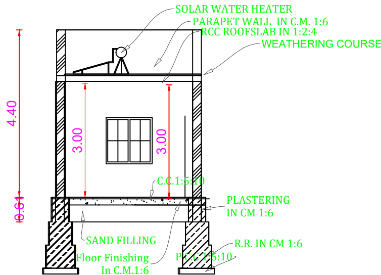
Section KV
