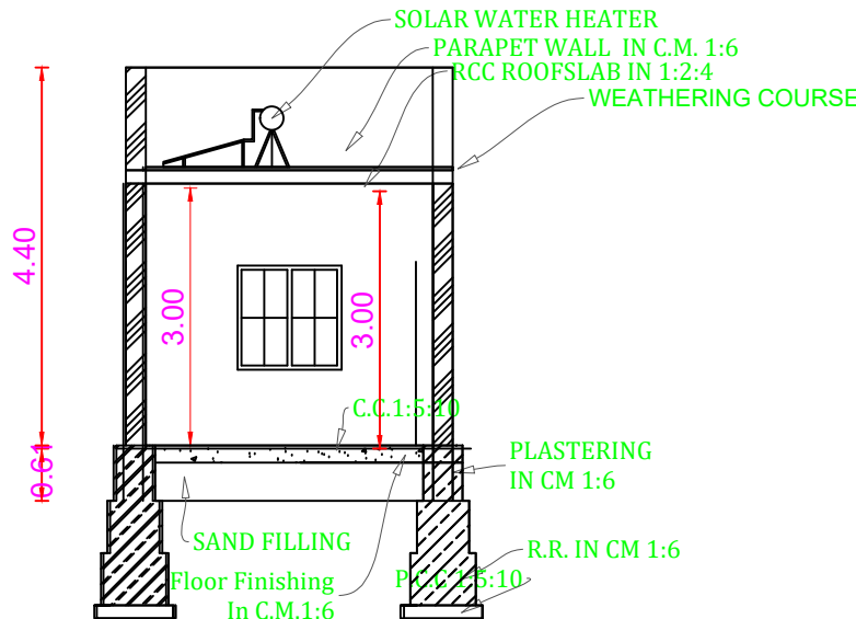
Section KV
