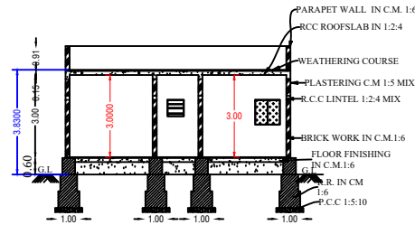
SECTION ON-"AB"
