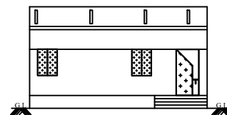
FRONT ELEVATION
