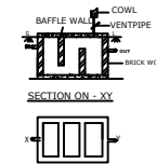
SEPTICTANK DETAILS
