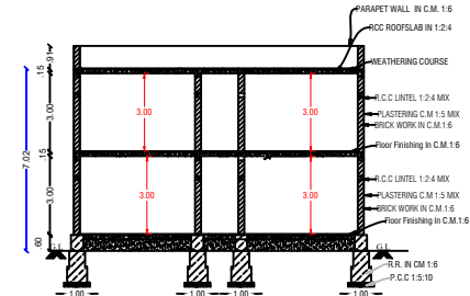
SECTION ON-"AB"
