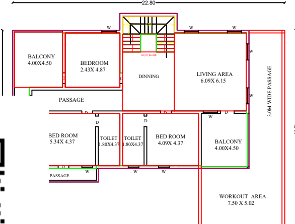
FRIST FLOOR PLAN
