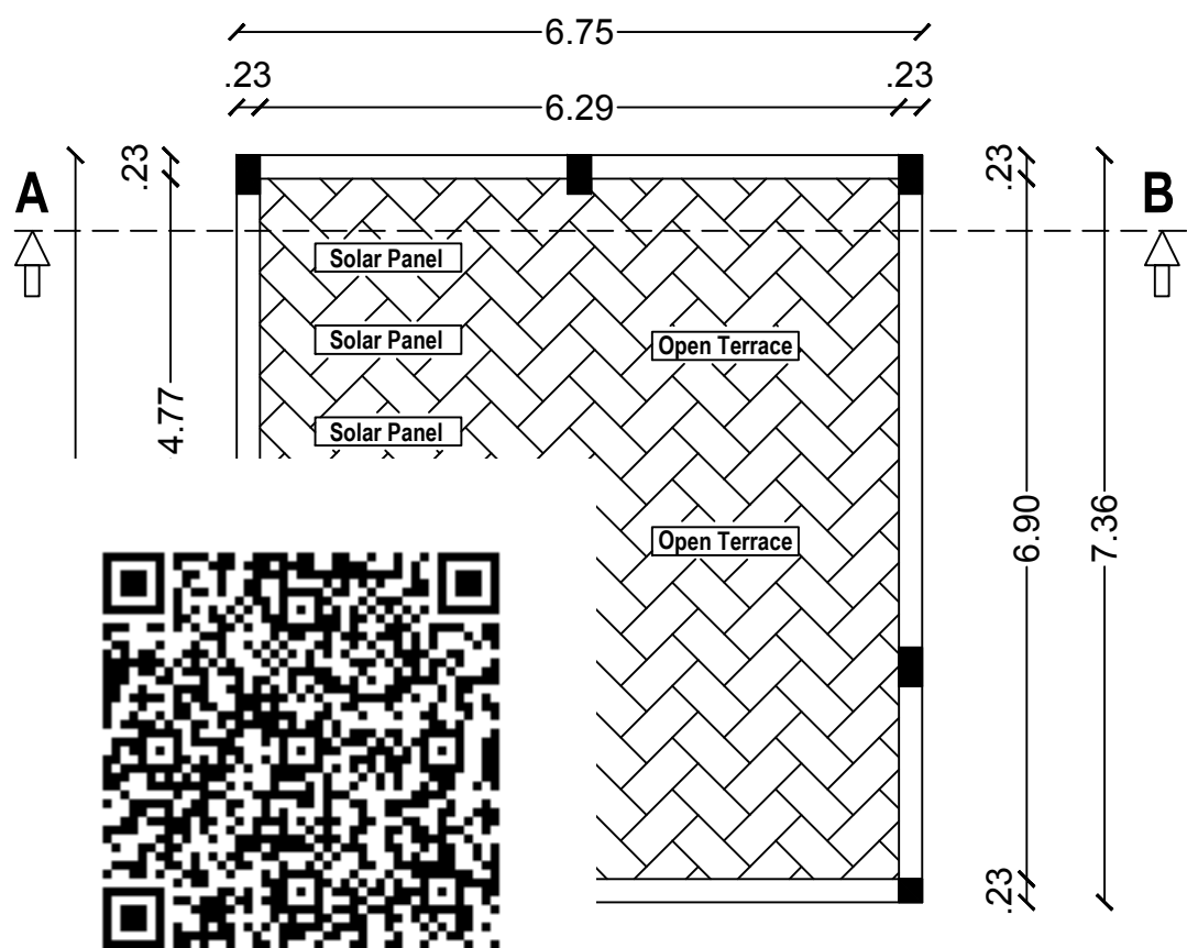
Floor Plan
