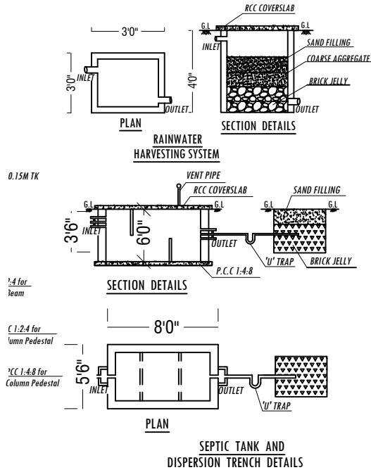
SEPTIC TANK AND DISPERSION TRENCH DETAILS
