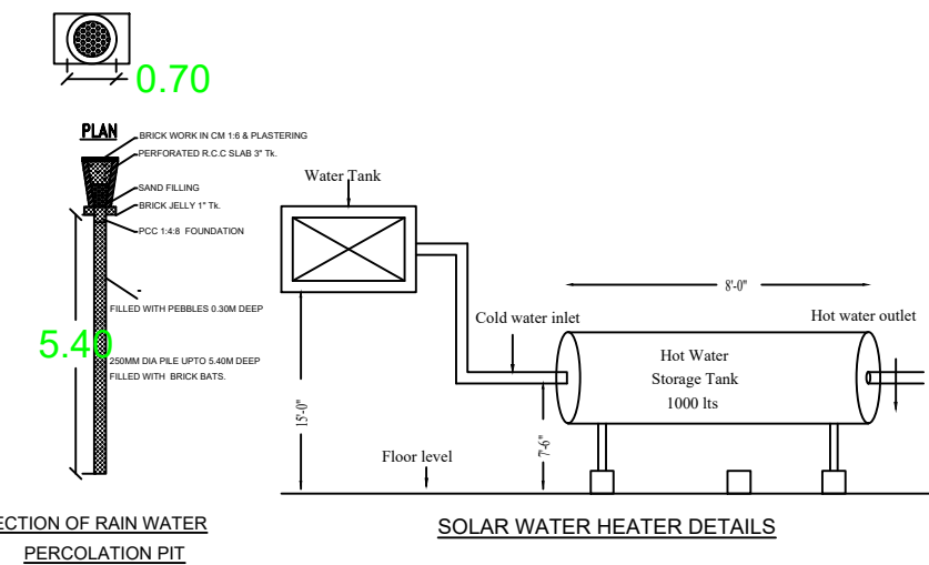
SOLAR WATER HEATER DETAILS
