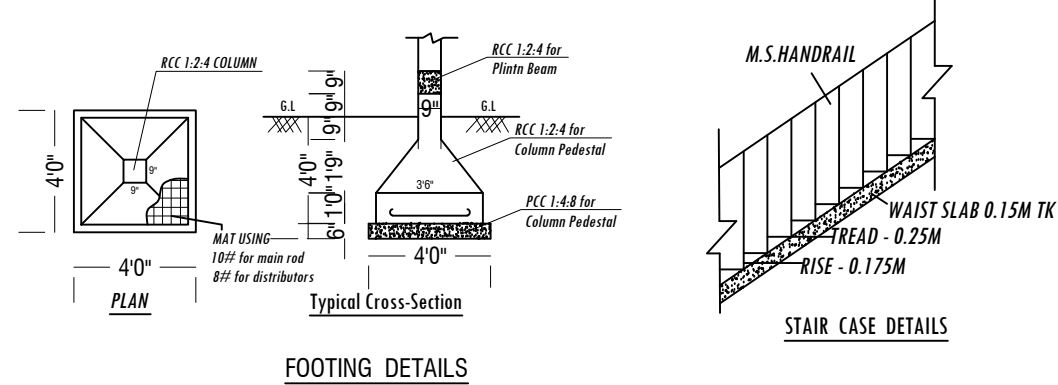
FOOTING DETAILS
