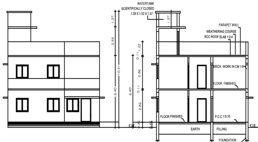
FRONT ELEVATION
