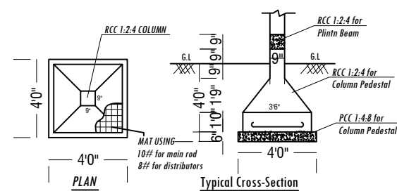
FOOTING DETAILS
