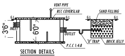
SECTION DETAILS
