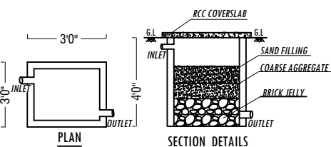
RAINWATER HARVESTING SYSTEM
